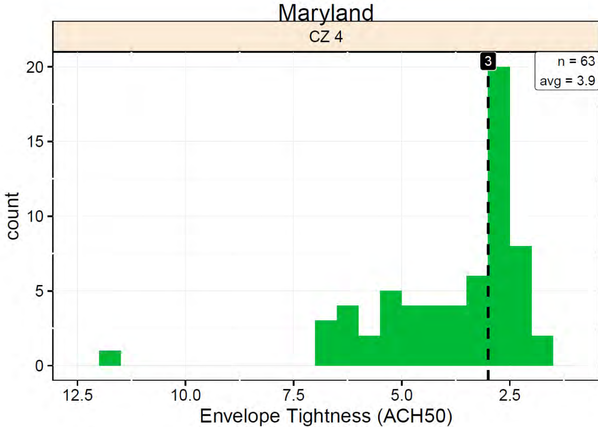
Figure 3.1. Envelope Tightness
